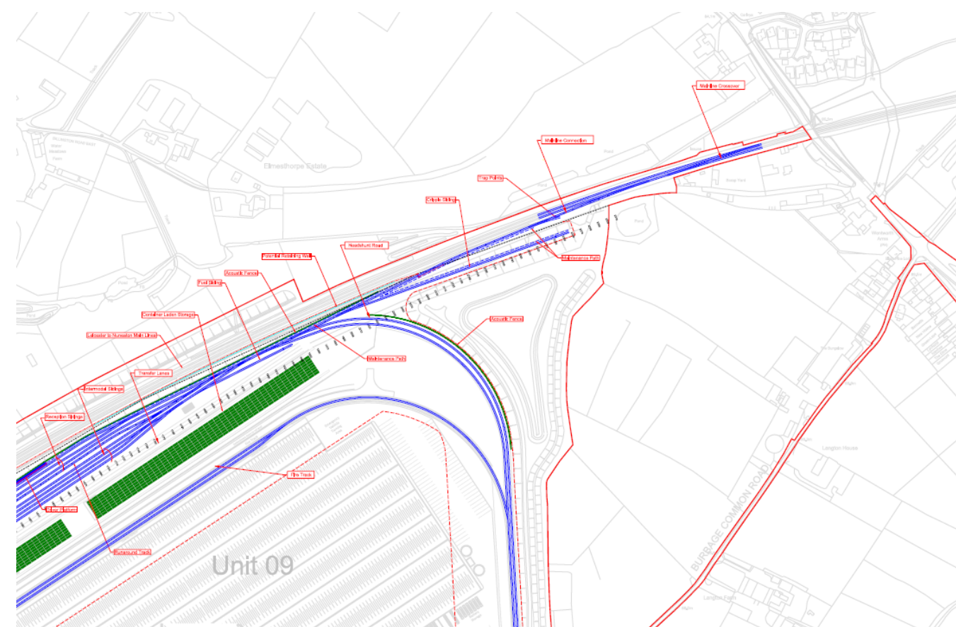
Fig 60. Eastern Arrangement of Main Reception sidings, intermodal sidings and container storage. Document Reference 2.25
