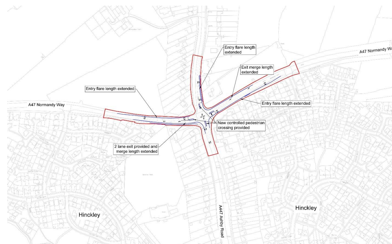
Fig 53. Proposed Works to the A47 / Ashby Road Junction, Hinckley (Document Reference 6.3.3.3)
