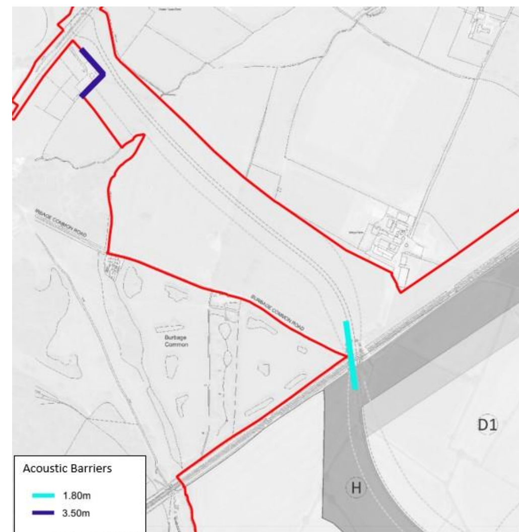
Fig. 65 Proposed Noise Barriers on new bridge on A47 Link road and adjacent to the junction with Leicester Road. (Document Reference 6.3.10.10)
