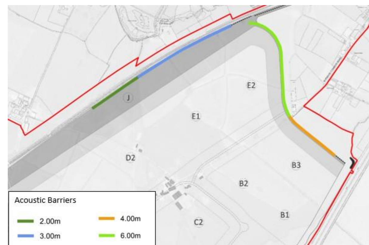
Fig. 63 Proposed Noise Barriers to north west of Railport and to the north east of head shunt (Document Reference 6.3.10.10)
